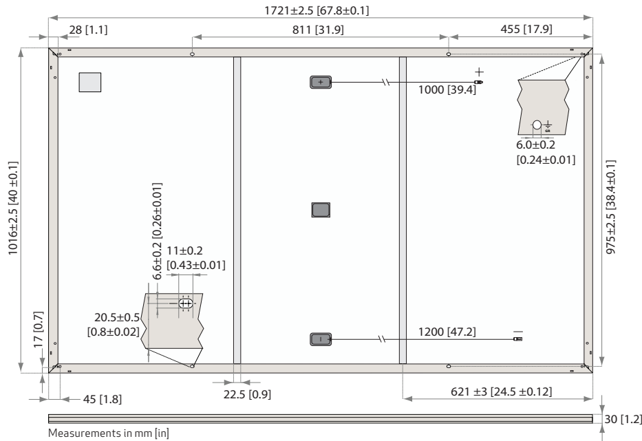
Fig. 18: Panel dimensions: REC Alpha Series
