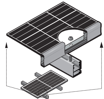
Fig. 14: Mounting hole installation example
